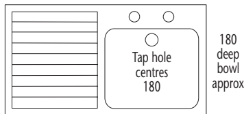
DBL(left) DBR(right) Single bowl, single drainer
