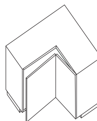
D121P Corner bifold door (right) H750 x W900 x W900 x D450
