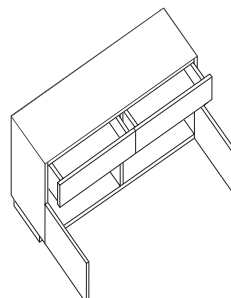
D65P Double drawer and door H750 x W1200 x D450
