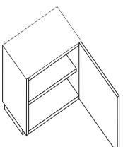
D110SP (left) D111SP (right) Single door left/right H750 x W600 x D450
