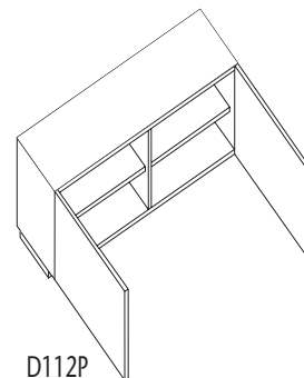
D112P Double door H750 x W1200 x D450
