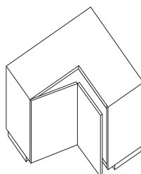
D120P Corner bifold door (left) H750 x W900 x W900 x D450
