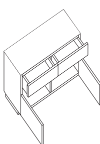
D64P Double drawer and door H750 x W1000 x D450
