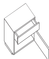
D62P (left) D63P (right) Single door/drawer left/right H750 x W600 x D450
