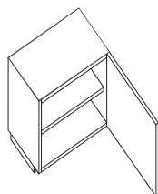
D110P (left) D111P (right) Single door left/right H750 x W600 x D450
