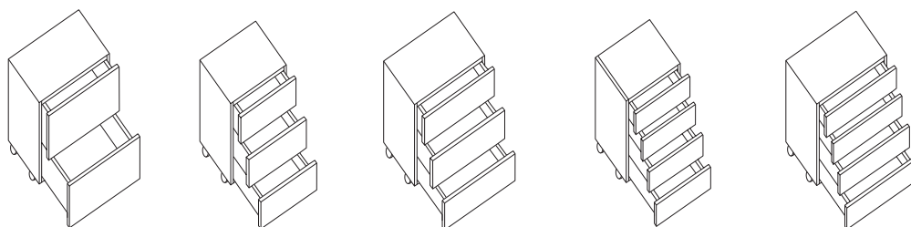
D95PM Filing 2 drawer H835 x W600 x D600
