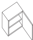
A15(right) Single door cupboard H550 x W500 x D300
