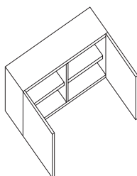
A17 Double door cupboard H550 x W1000 x D300
