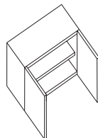
A16 Double door cupboard H550 x W600 x D300
