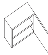
A31 Single door cupboard H550 x W600 x D300
