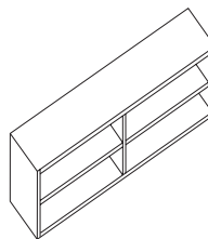
A320 Open wall unit H550 x W1200 x D300
