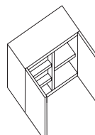
A20 Urine test cupboard, lockable H550 x W600 x D300
