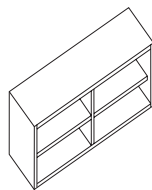
A170 Open wall unit H550 x W1000 x D300
