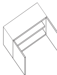
D80SC Double door H550 x W1000 x D450
