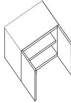
D79C Double door H550 x W600 x D450
