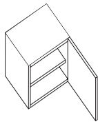
D75C(left) D76C(right) Single door left/right H550 x W500 x D450
