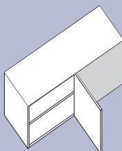
D122C Corner single door (left) H550 x W900 x D450
