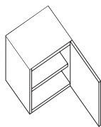
D75SC(left) D76SC(right) Single door left/right H550 x W500 x D450
