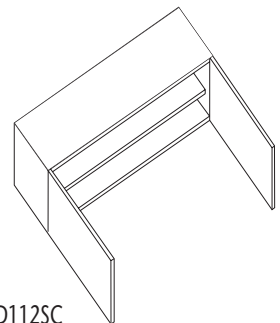
D112SC Double door H550 x W1200 x D450
