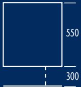
D60C(left) D61C(right) Single door/drawer left/right H550 x W500 x D450
