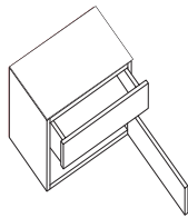
D62C(left) D63C(right) Single door/drawer left/right H550 x W600 x D450
