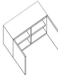
D80C Double door H550 x W1000 x D450
