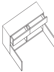
D64C Double drawer and door H550 x W1000 x D450
