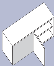
D123C Corner single door (right) H550 x W900 x D450
