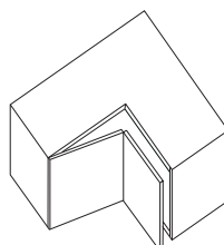
D120C Corner bifold door (left) H550 x W900 x D450
