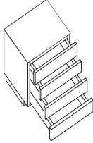
D102/4CP Four drawer H550 x W500 x D450
