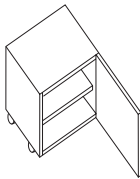
D75CM(left) D76CM(right) Single Door H635 x W500 x D600
