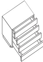
D103/4CP Four drawer H550 x W600 x D450
