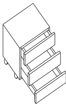
D102/3CM Three drawer H635 x W500 x D600
